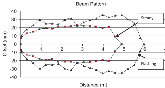
Fig. 7. Optical Sensor. Field of View from Experiment
