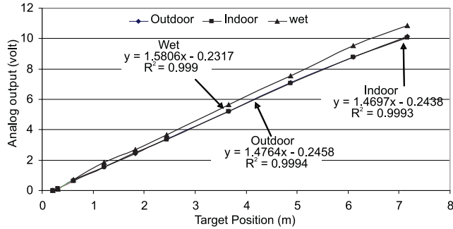
Fig. 6. Ultrasonic Sensor characteristics-Sensing range vs. voltage output in different conditions
