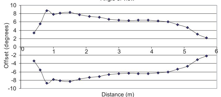
Fig. 5. Angle of view for the Banner ultrasonic sensor
