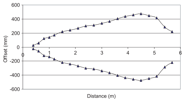
Fig. 4. Ultrasonic Sensor. Field of View from Experiment
